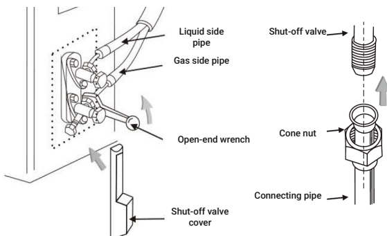
Connection Pipe Installation
